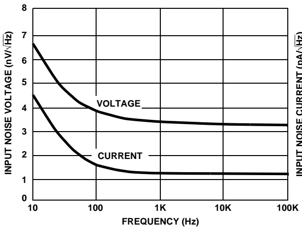
FIGURE 6. NOISE SPECTRUM
